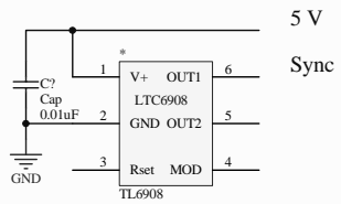
Alternative spread spectrum oscillator
